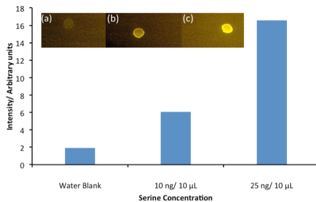
Figure 5: Luminescence intensity of amino acid spots on paper developed with DMAF ( \lambda_{ex} = 505 nm, \lambda_{em} = 580 nm) (a) water blank (b) 10 ng/10 \mu L serine (c) 25 ng/10 \mu L serine
