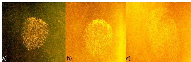
Figure 3: Fingerprints developed with varying concentrations of DMAF in 100mL of hexane. The background luminescence greatly increases with the concentration (a) 20 mg/100 mL (b) 80 mg/100 mL (c) 160 mg/100 mL
