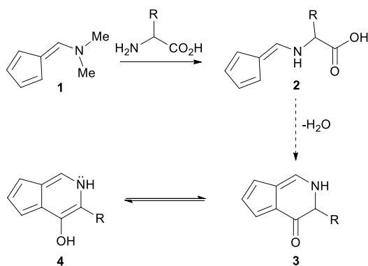
Scheme 1: Proposed reaction mechanism of DMAF with amino acids
