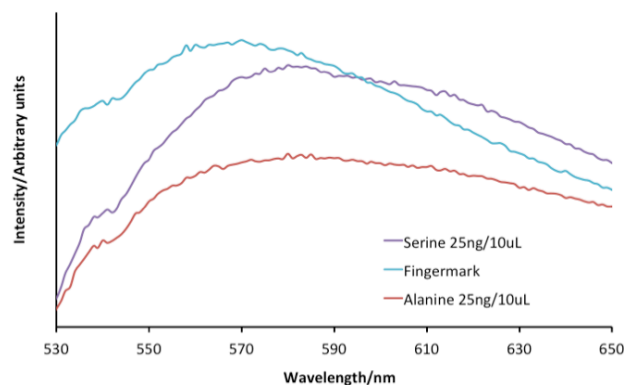
Figure 6: Fluorescence spectra of amino acid spots and a latent fingerprint on paper developed with DMAF ( \lambda_{ex} = 505 nm)
