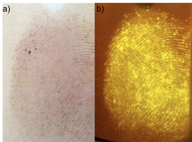
Figure 1: 6-(N,N)-(dimethylamino)fulvene treated latent fingerprint. Images were taken with a Nikon D100 SLR (85 mm focal length, ISO 200): a) absorbance mode (shutter speed 1/30 s and aperture f9); b) photoluminescence mode with excitation using a Polilight PL 500 at 505 nm and viewed through a KV 550 filter, (shutter speed 1 s, aperture f9).
