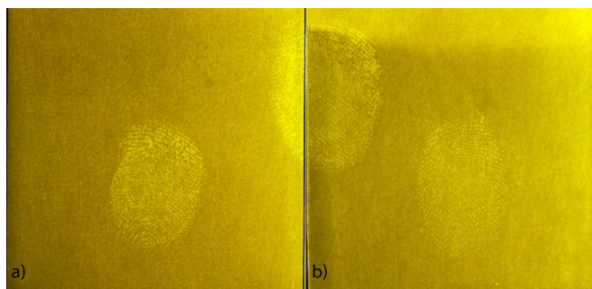
Figure 2: Comparison of HFE-7100 and Hexane when used as a carrier solvent. The fingerprints are from the same donor on the same hand, cut in half down the middle (a) HFE-7100 (b) hexane
