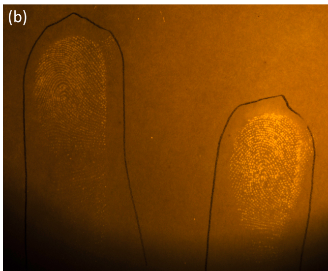
Figure 4: 6-(N,N)-(dimethylamino)fulvene treated latent fingerprints. Images were taken with a Nikon D300 SLR (60 mm focal length, ISO 200): a) absorbance mode (shutter speed 1/40 s and aperture f8); b) photoluminescence mode with excitation using a Polilight PL 500 at 505 nm and viewed through a KV 550 filter, (shutter speed 1/15 s, aperture f8)
