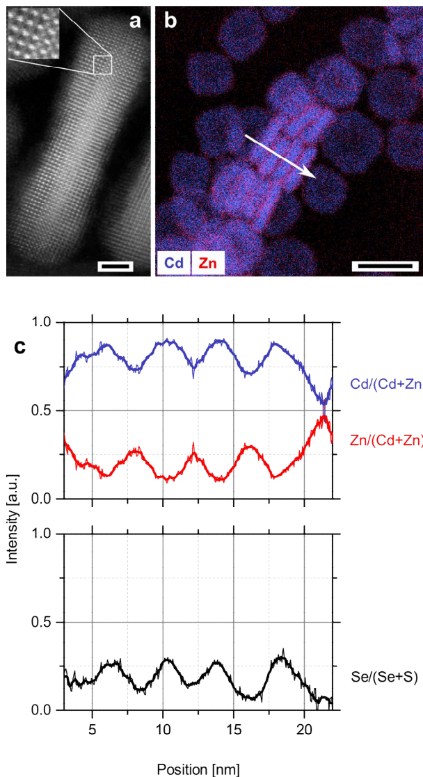
Figure 5. Structural analysis of the CdSe/Cd x Zn 1-x S core/shell NPLs shown in Figure 1c. (a) High-resolution HAADF STEM cross-sectional image of a single core/shell NPL. The brighter core can be distinguished from the darker shell due to the higher atomic number of the core elements. (b) Superposition of energy-dispersive X-ray spectrographs (EDS) of Cd and Zn for NPLs seen in top- and side-view. (c) The corresponding concentration profile across four vertically stacked NPLs, observed from the side. The collection area is marked with the white arrow in (b). Note that a single core/shell NPL in top-view is detected on the left of the stacked NPLs at positions between 0 and ~7 nm in (c). Black scale bars are 2 nm in (a) and 20 nm in (b).
