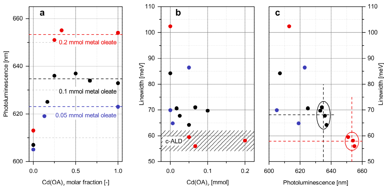
Figure 4. Influence of the precursor ratio and total precursor concentration on the emission properties of CdSe/Cd x Zn 1-x S NPLs. Blue, black, and red dots correspond to reaction series with 0.05, 0.1, and 0.2 mmols of total metal oleate [Cd(OA) 2 + Zn(OA) 2 ], respectively. (a) Evolution of the emission wavelength as a function of the Cd(OA) 2 molar fraction (relative to the total amount of metal oleate) during the shell growth. (b) Influence of the concentration of Cd(OA) 2 on the emission linewidth. The shaded area indicates the linewidth range reported for CdSe/CdS core/shell NPLs synthesized by colloidal atomic layer deposition (c-ALD). 20-21 (c) Relation between the emission wavelength and the corresponding linewidth. The dashed lines indicate the mean photoluminescence wavelengths and linewidths for the reactions using a Cd(OA) 2 molar fraction ≥ 25% (data points inside the circles).
