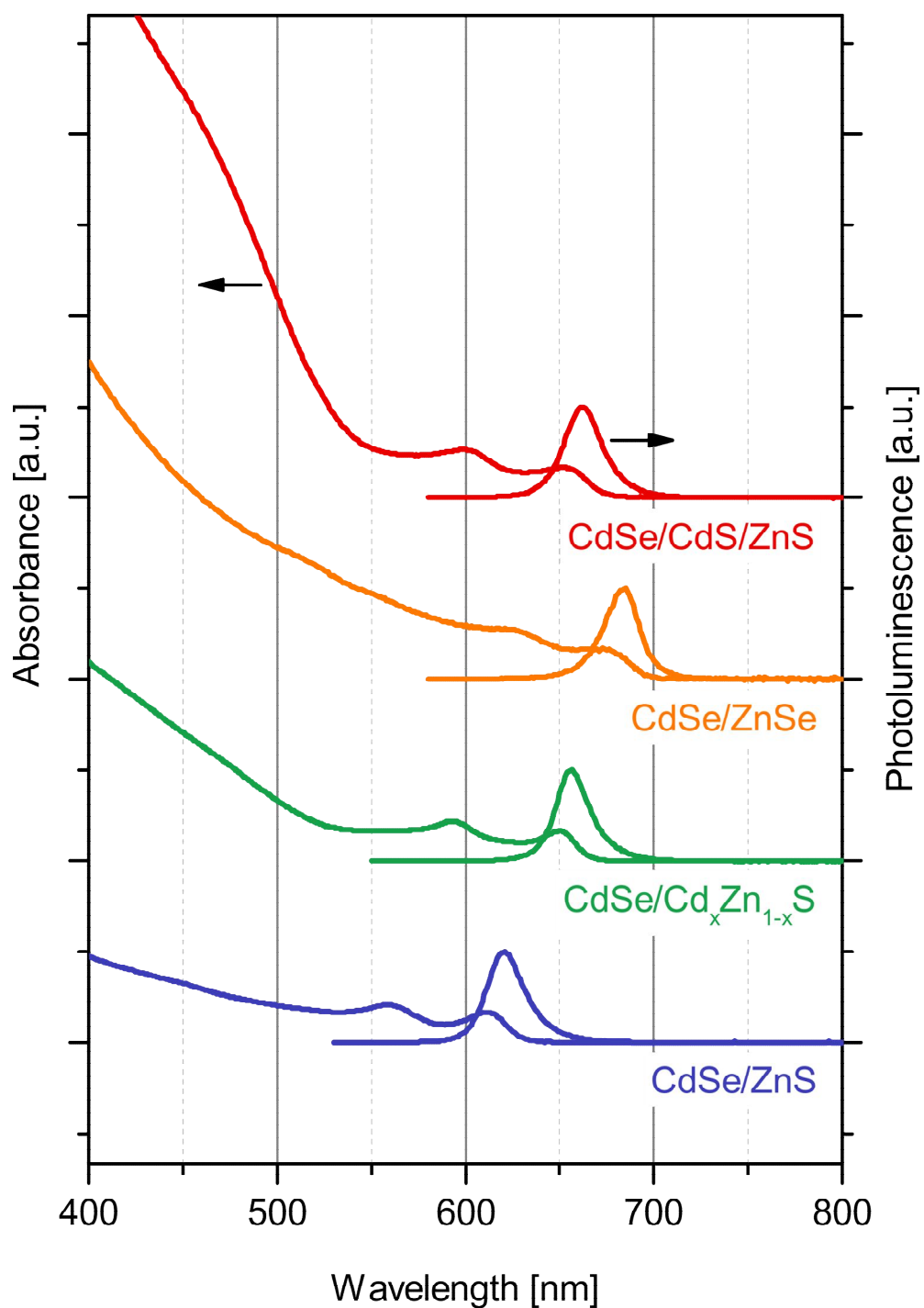
Figure 3. Optical absorption and emission spectra for the core/shell NPLs shown in Figure 1. The emission linewidths range from 56 meV for CdSe/Cd x Zn 1-x S to 76 meV for CdSe/ZnS core/shell NPLs (see Table S1 in the Supporting Information for all parameters).
