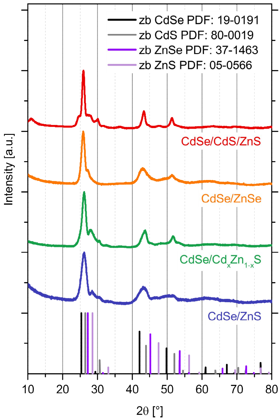
Figure 2. Powder X-ray diffraction (XRD) patterns for the core/shell NPLs shown in Figure 1. Reference patterns (labelled by their powder diffraction file, PDF) are shown for zinc blende crystals of CdSe, CdS, ZnSe, and ZnS.
