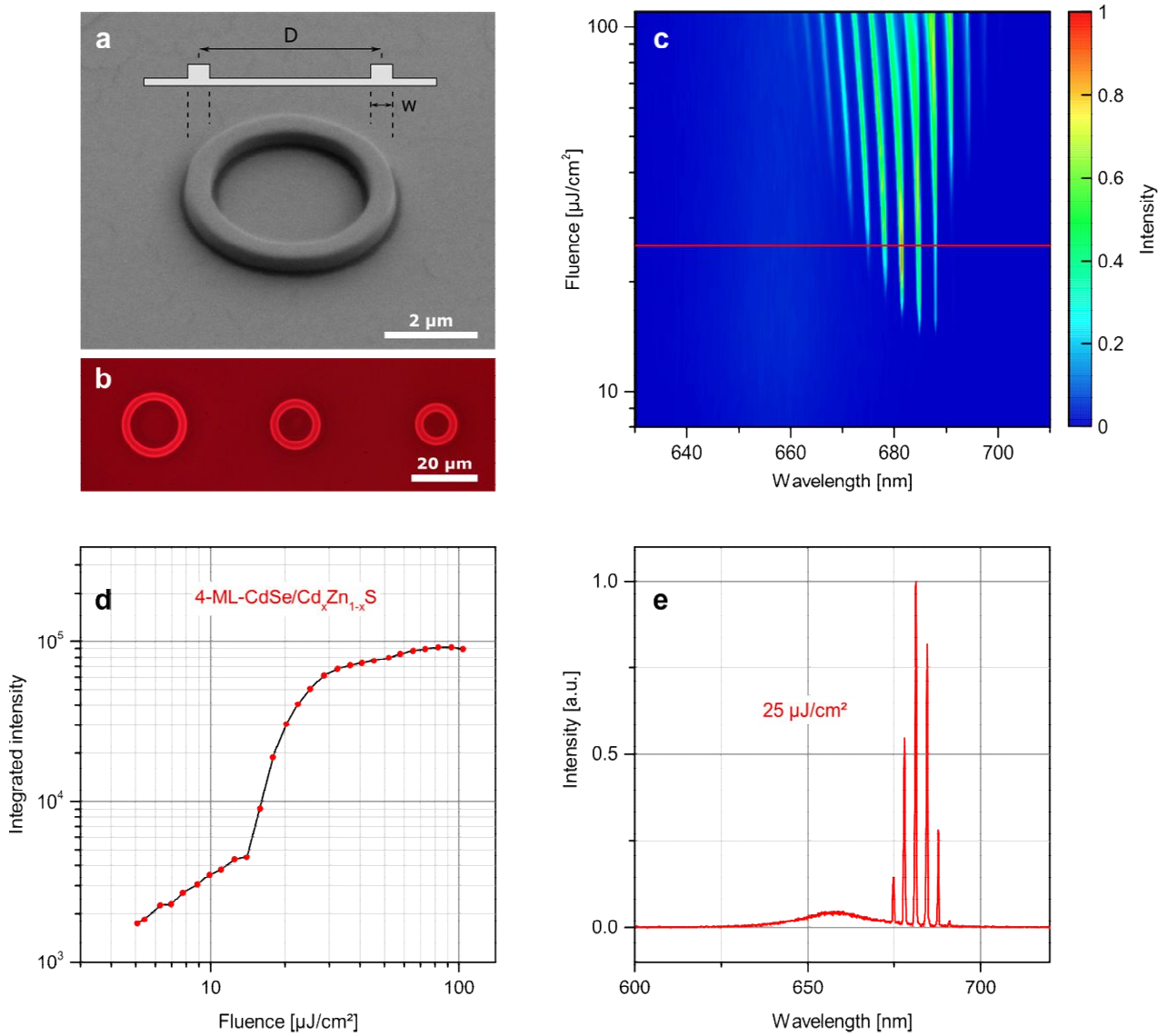
Figure 7. 4-monolayer-CdSe/Cd x Zn 1-x S core/shell NPL ring resonators and their optical characterization for lasing. (a) Scanning electron micrograph (SEM) of a template-stripped NPL ring resonator. The inset shows a cross-sectional schematic of the ring structure. Rings were fabricated with variable diameters ( D ) and widths ( w ) and a height of \sim 500 nm. (b) Fluorescence image of ring resonators of varying diameters illuminated with ultraviolet light. (c) Power-dependent emission spectra collected from a ring with D = 20\ \mu\text{m} and w = 1\ \mu\text{m} . Narrow lasing lines evolve at fluences above a threshold of 13\ \mu\text{J}/\text{cm}^2 . (d) Corresponding emission intensity integrated over all collected wavelengths and averaged over the area of the ring resonator versus the excitation fluence. (e) Emission spectrum under lasing conditions extracted at a power of 25\ \mu\text{J}/\text{cm}^2 [indicated with a red horizontal line in (c)].
