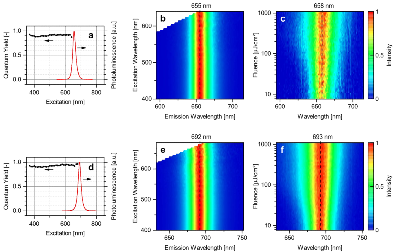
Figure 6. Room-temperature excitation-dependent photoluminescence characterization of CdSe/Cd x Zn 1-x S core/shell NPLs having CdSe cores with a thickness of 4 monolayers (a-c) and 6 monolayers (d-f). (a,d) Photoluminescence quantum yields (QYs) measured at different excitation wavelengths. The corresponding emission spectra are shown in red. (b,e) Normalized photoluminescence excitation–emission spectra of core/shell NPL dispersions in hexane. The black vertical dashed lines at 655 nm (b) and 692 nm (e) are added for visualization. (c,f) Normalized photoluminescence emission spectra of core/shell NPL films versus the excitation fluence (405 nm excitation, ~340 fs pulse duration, 10 kHz repetition rate). The black vertical dashed lines at 658 nm (b) and 693 nm (c) are added for visualization.
