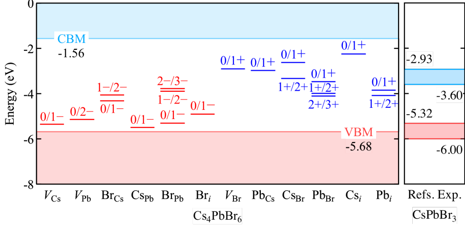
Figure 2: The natural electronic band alignment with respect to vacuum level (set to 0 eV). Range of reported CsPbBr 3 valence band maximum (VBM) and conduction band minimum (CBM) values are shown for comparison as taken from Refs. 32–35. The thermodynamic defect transition levels for each point defect are marked in red (acceptor defect) and blue (donor defect) dashes with respect to the valence and conduction bands of Cs 4 PbBr 6 .
