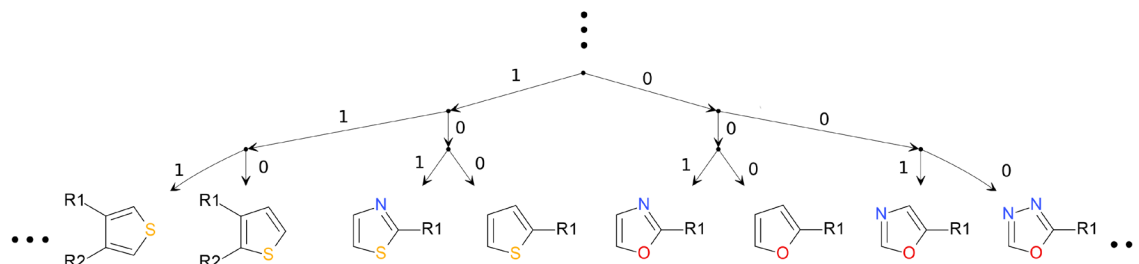
Figure 2. A sub-part of the binary tree holding all fragments. It can be seen that fragments that are similar to each other are placed close to each other in the tree. The encoding of a fragment is determined by the path from the root to the leaf where the fragment is stored. Every branching to the left will add a 1 to the end of the encoding and every branching to the right will add a 0. The attachment points of the fragments are marked with an R and the number of the order in which they will bind.
