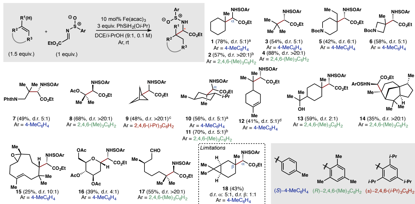
Figure 2. Alkyl radicals generated by MHAT add to chiral sulfinimines. d.r. of two major diastereomers reported. a stereochemistry at the \alpha -carbon is ( S ). b stereochemistry in the \alpha -carbon is ( R ). c Mn(dpm) 3 instead of Fe(acac) 3 was used. d contains 15% unrearranged pinene product and its diastereomer.
