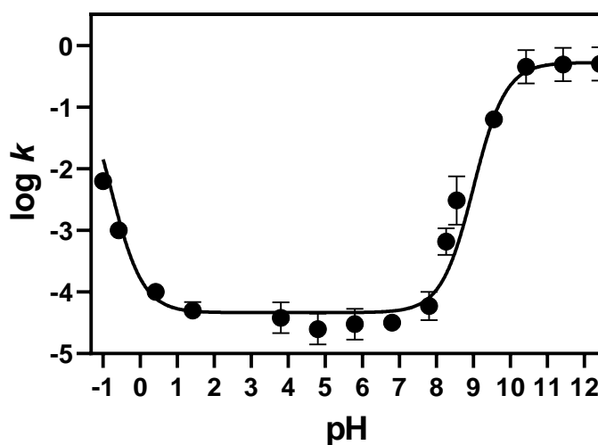
Fig. 2. pH-rate constant profile for hydrolysis of PNPGLc, corrected for pH at 90 °C. k_{\text{H}} = 2.90 \times 10^{-3} \text{ M}^{-1} \text{ min}^{-1} , k_{\text{uncat}} = 3.77 \times 10^{-5} \text{ min}^{-1} , k_{\text{OH}} = 5.82 \times 10^{-2} \text{ M}^{-1} \text{ min}^{-1} , k_{\text{NGP}} = 0.27 \text{ min}^{-1} (for rate data, see Table S15 ).
