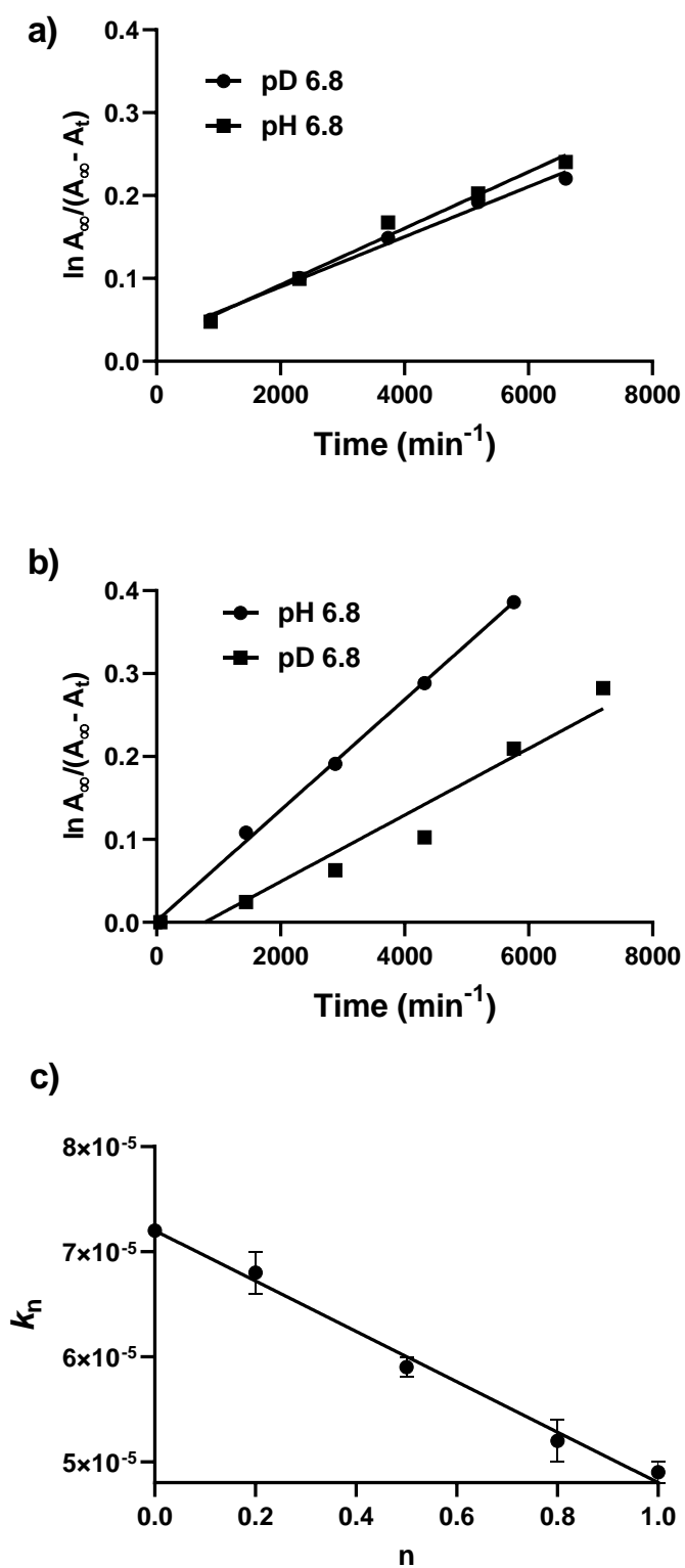
Fig. 3. Reactions in the pH independent region (pH = 6.8) at 90 °C. (a) Solvent isotope effect at [buffer] = 0.005 M. (b) Solvent isotope effect for [buffer] = 1 M. (c) Proton inventory plot of k_n as a function of D_2O fraction ( n ) at [buffer] = 1 M, p(H,D) 6.8.
